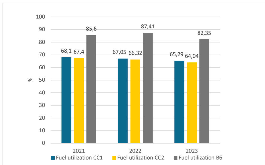
Figura 16 - Fuel utilization
